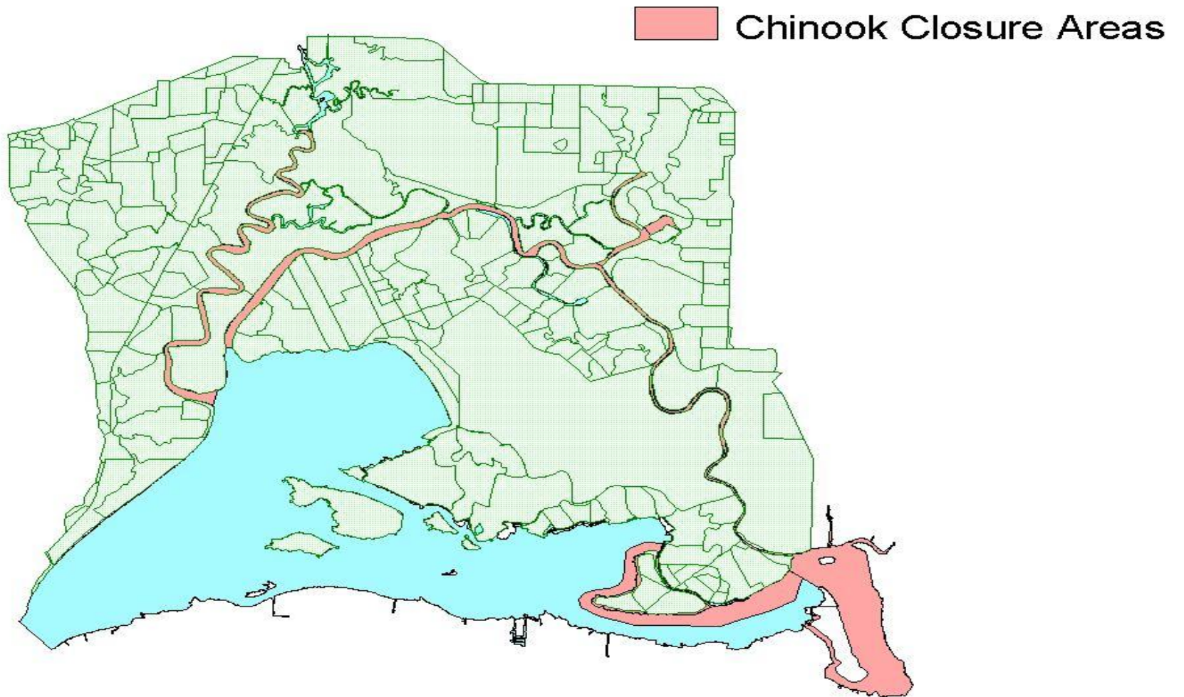
Figure D-2. Suisun Marsh Chinook Salmon Intake Closure Areas.
